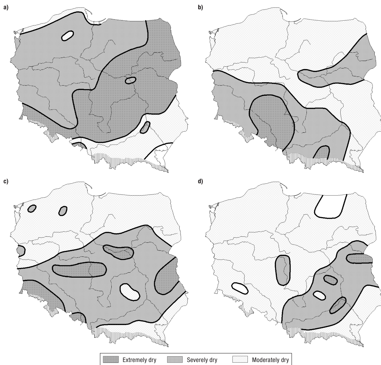
Figure 5. Spatial diversity of the occurrence of atmospheric drought in Poland in chosen years and development stages of cucumber: a, BF-BH in 1971; b, EE-BF in 1976; c, EE-BF in 1994; d, S-EE in 1999. For period explanations see Figure 2.
