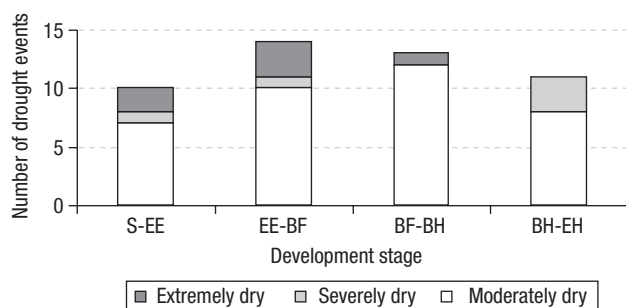
Figure 2. Average number of cases of the occurrence of atmospheric drought of different intensity (1966-2005) in the successive development stages of cucumber in Poland. S-EE: sowing-end of emergence. EE-BF: end emergence-beginning of flowering. BF-BH: beginning of flowering-beginning of harvesting. BH-EH: beginning of harvesting-end of harvesting.
